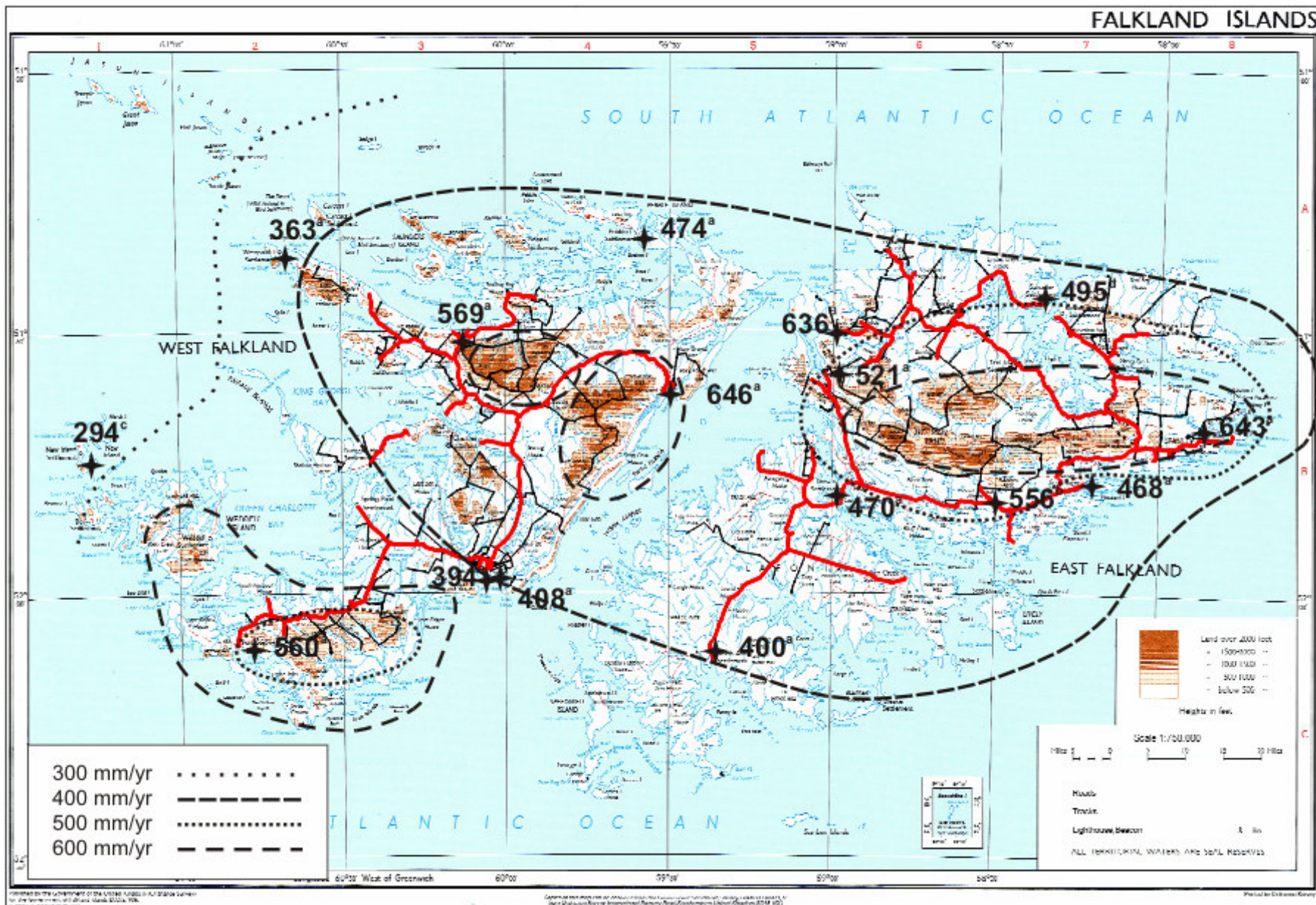
Figure 1.2. Relief map of the Falkland Islands ( after showing estimated zones of precipitation derived from historical data. Key: + measured precipitation means (mm/yr) and data sources for specific locations. Data sources: a. ; b. ; c. I. Strange, New Island South Conservation Trust (Pers. Comm.), d. Summers 7 McAdam (1993)
